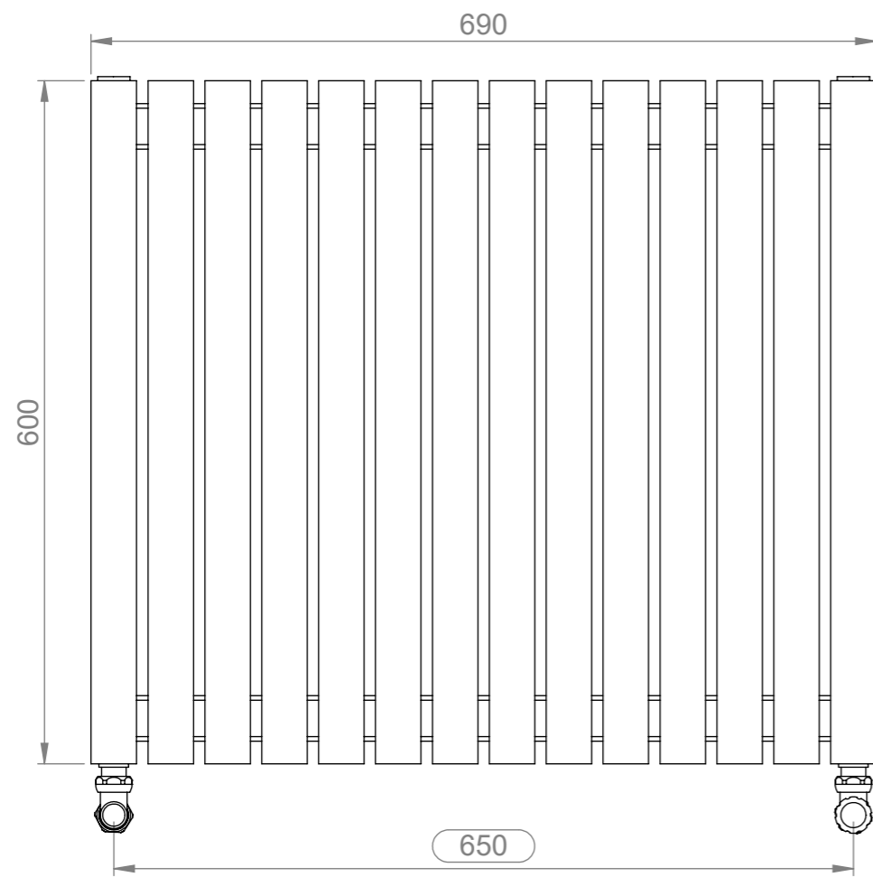
Front View
