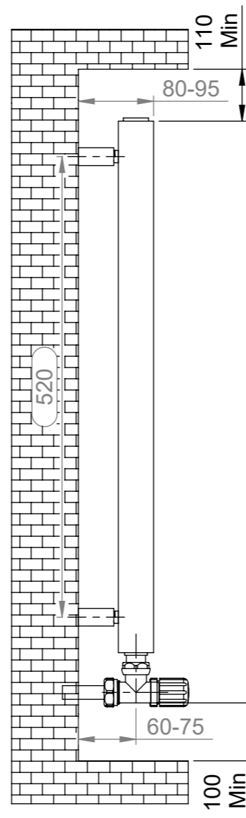
Side View
