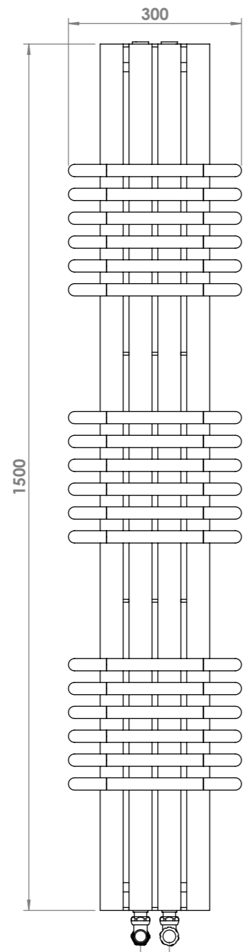
Front View
