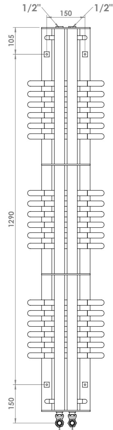
Back View
