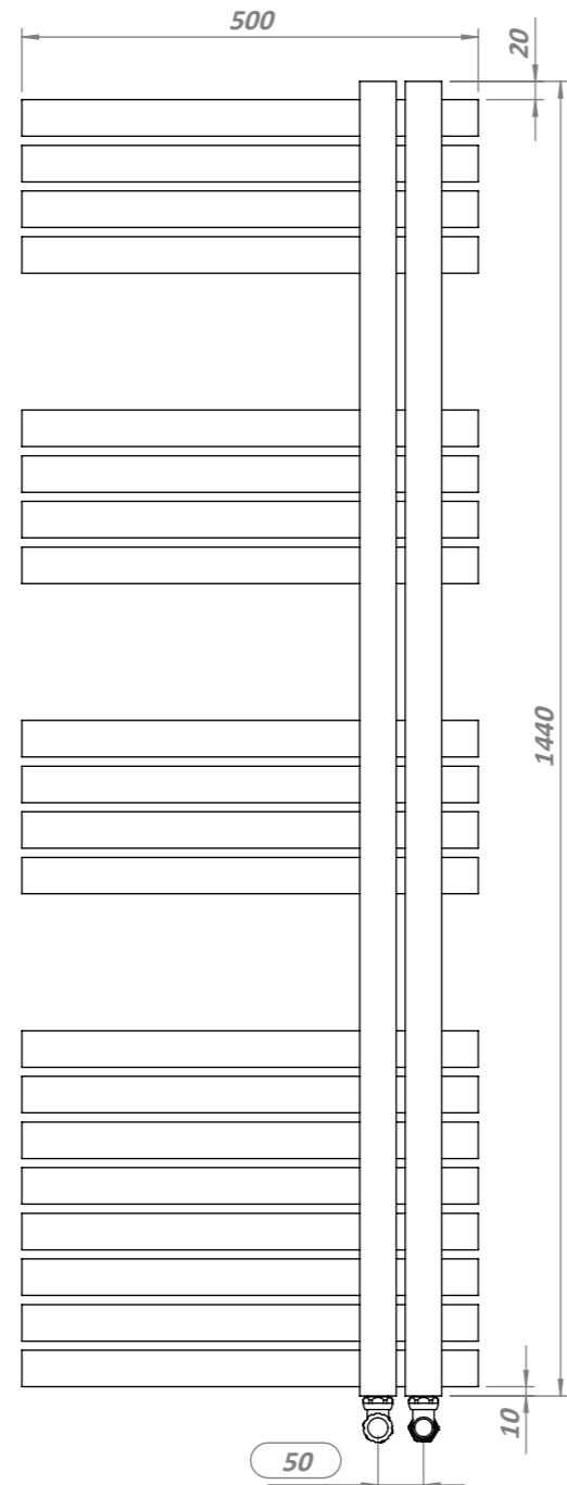
Front View
