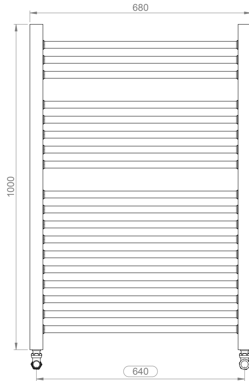
Front View
