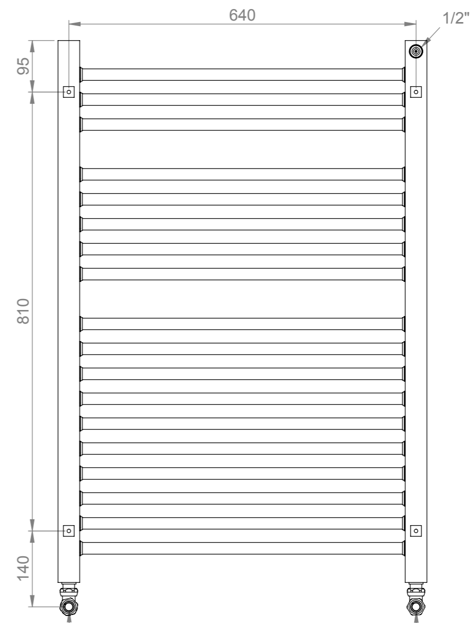
Back View
