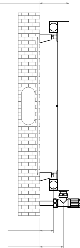
Side View
