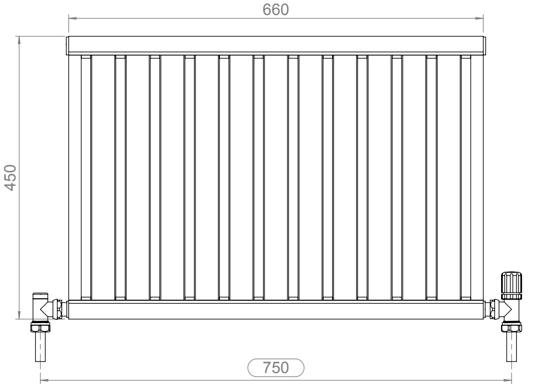
Front View
