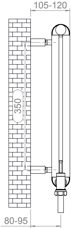
Side View
