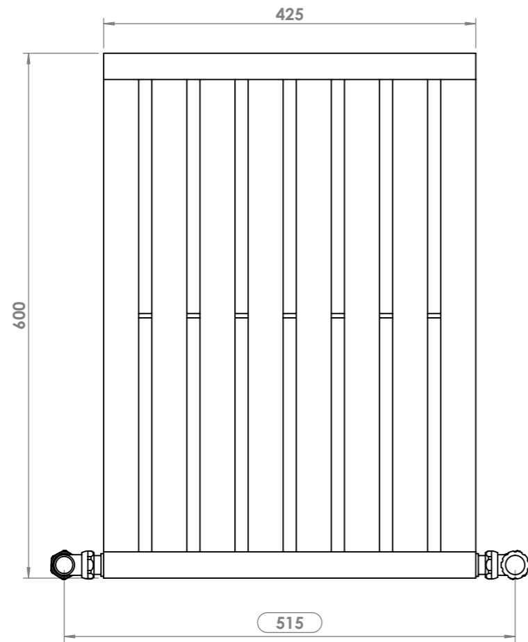
Front View
