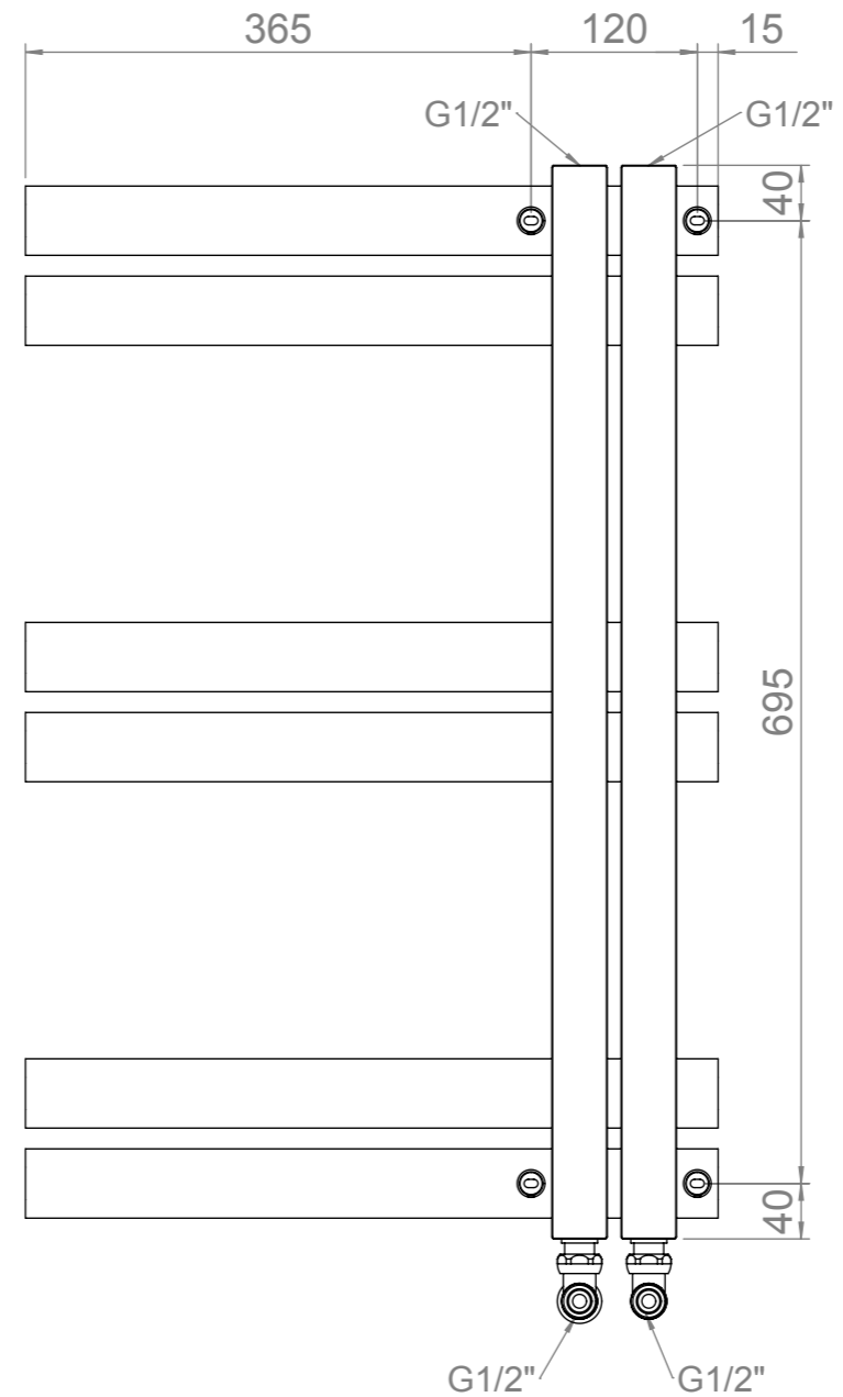
Back View
