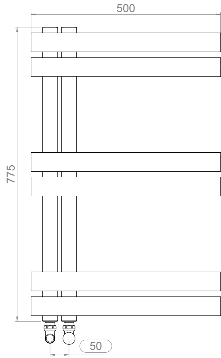
Front View
