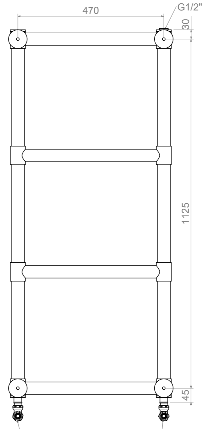
Back View
