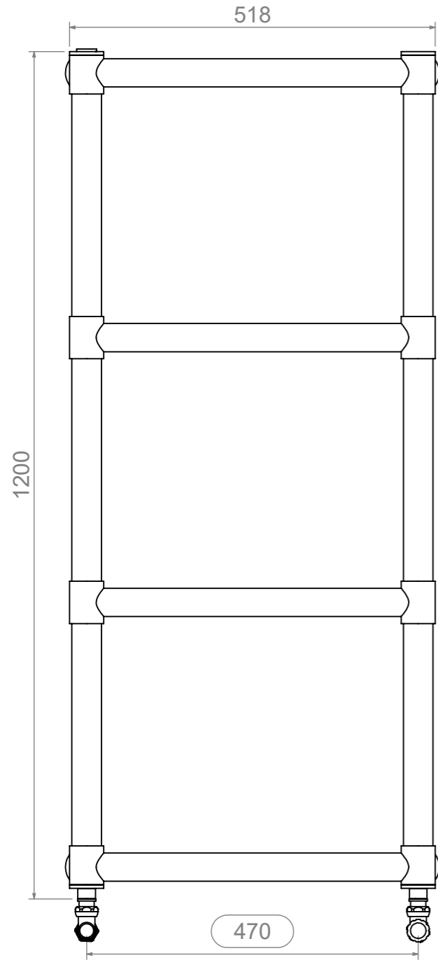
Front View
