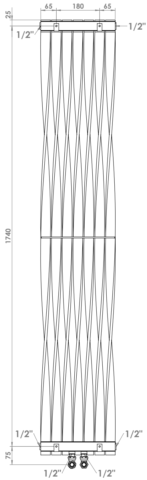
Back View
