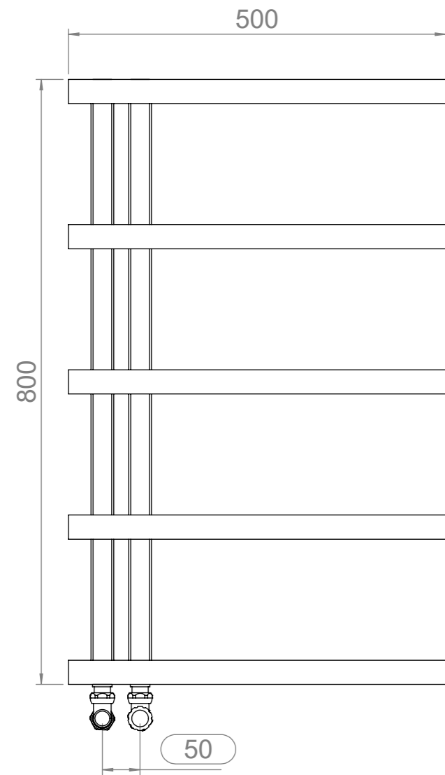
Front View
