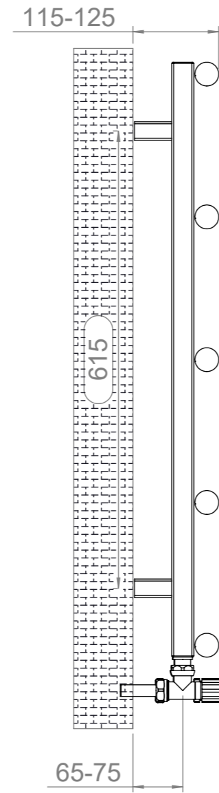
Side View
