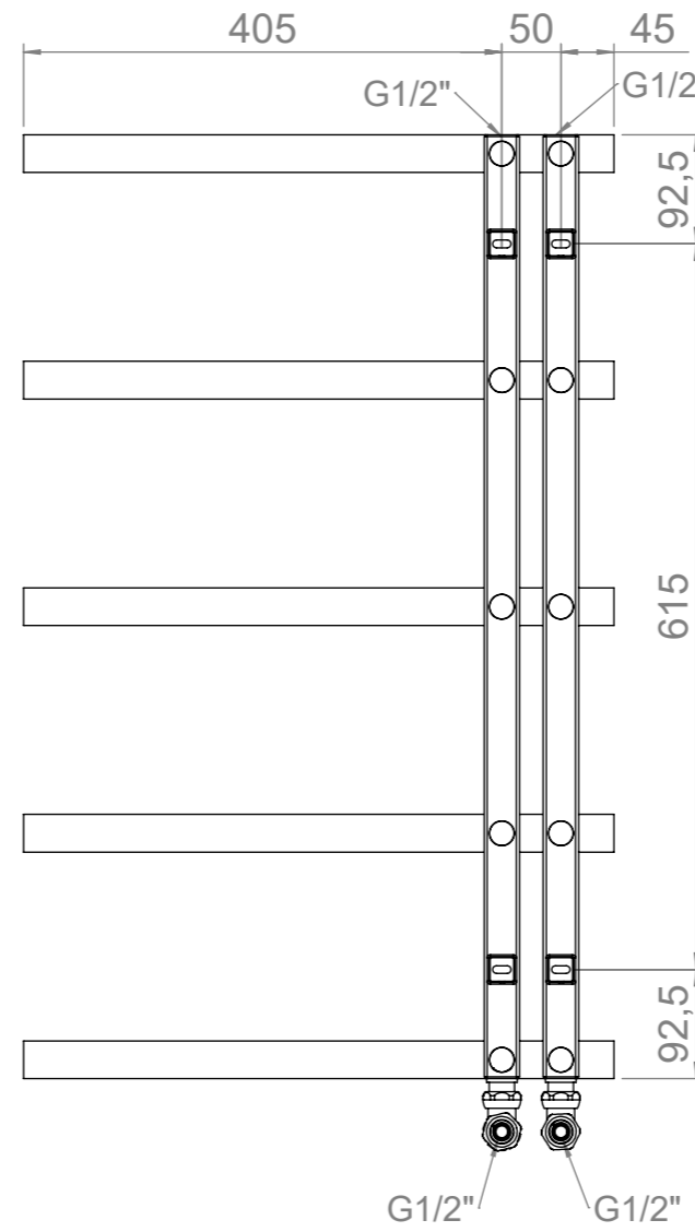
Back View
